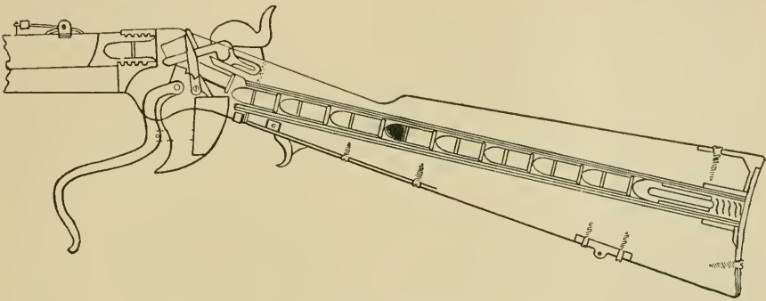
SPENCER CARBINE.
